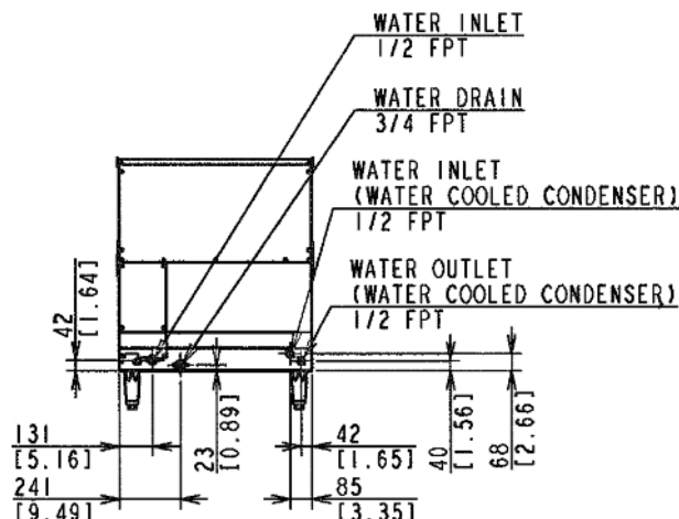
BACK VIEW / AIR-COOLED UNIT
